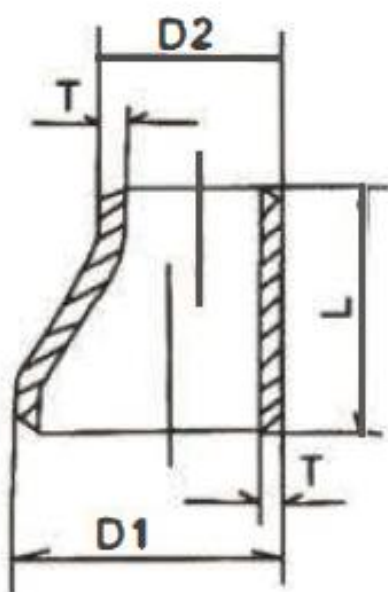
无缝偏心异径接头 Seamless Eccentric Special Joint
