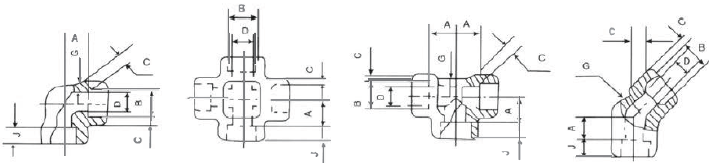
钢制承插焊管件STEEL SOCKET-WELDING FITTINGS 90° Elbows ) 四通 ( cross ) 三通 ( tees ) 45° 弯头 ( 45° Elbows )
