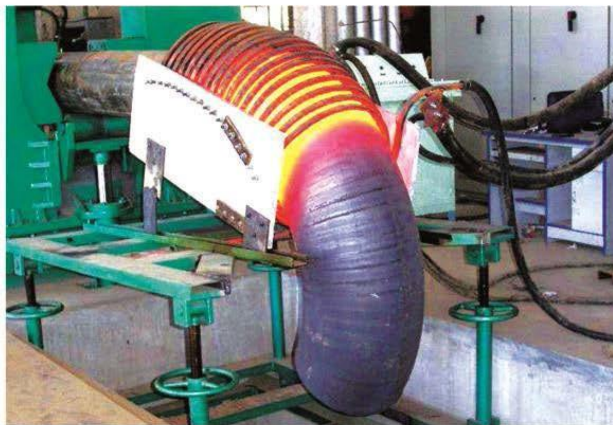
弯头推制机 ( Elbow push processing )
