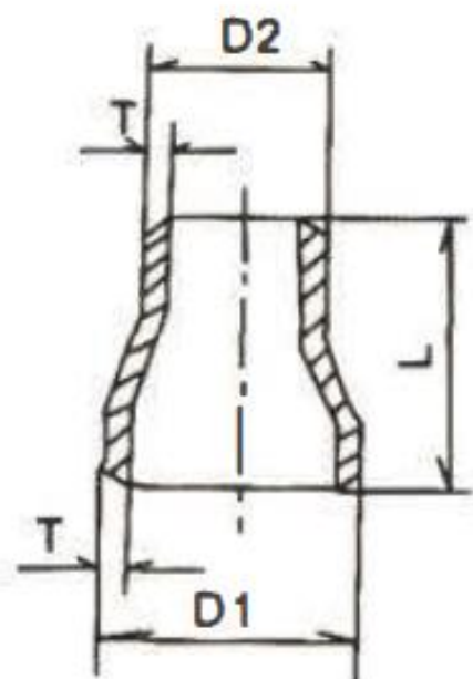
无缝同心异径接头 Seamless Cxoncentric Special Joint
