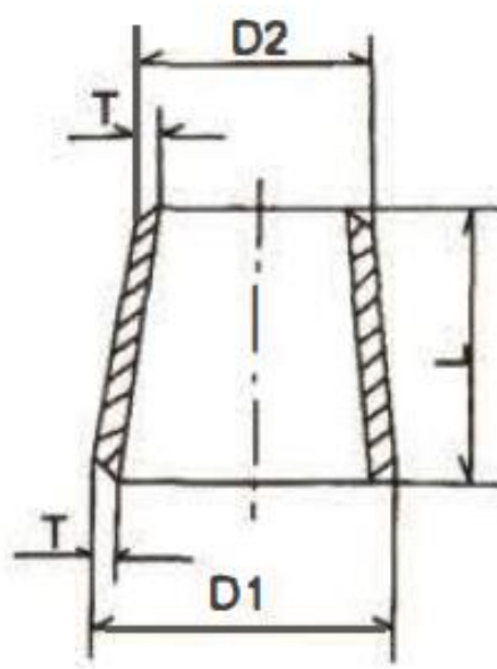
焊制同心异径接头 Welded Concentric Special Joint
