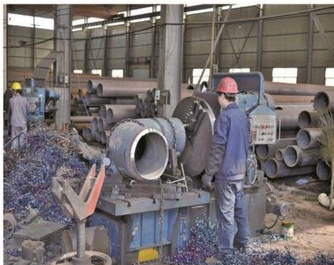
电动坡口机 ( Electric beveling machine )
