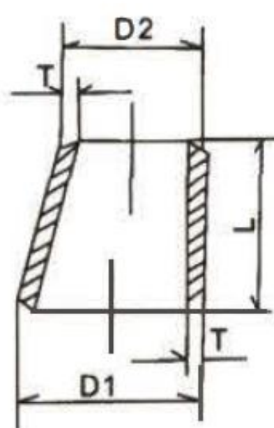
焊制偏心异径接头 Welded Eccentric Special Joint
