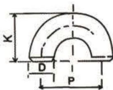
180° 弯头 Elbows
