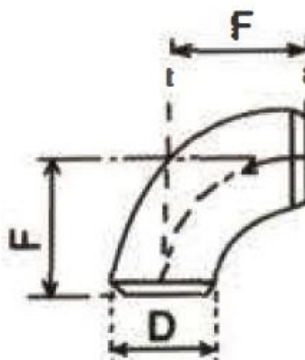
90° 弯头 Elbows
