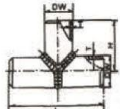
无缝焊接三通 Seamless welded tees (GD87)
