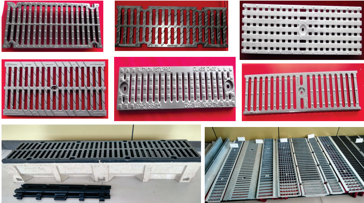
Channel grating as per EN1433
