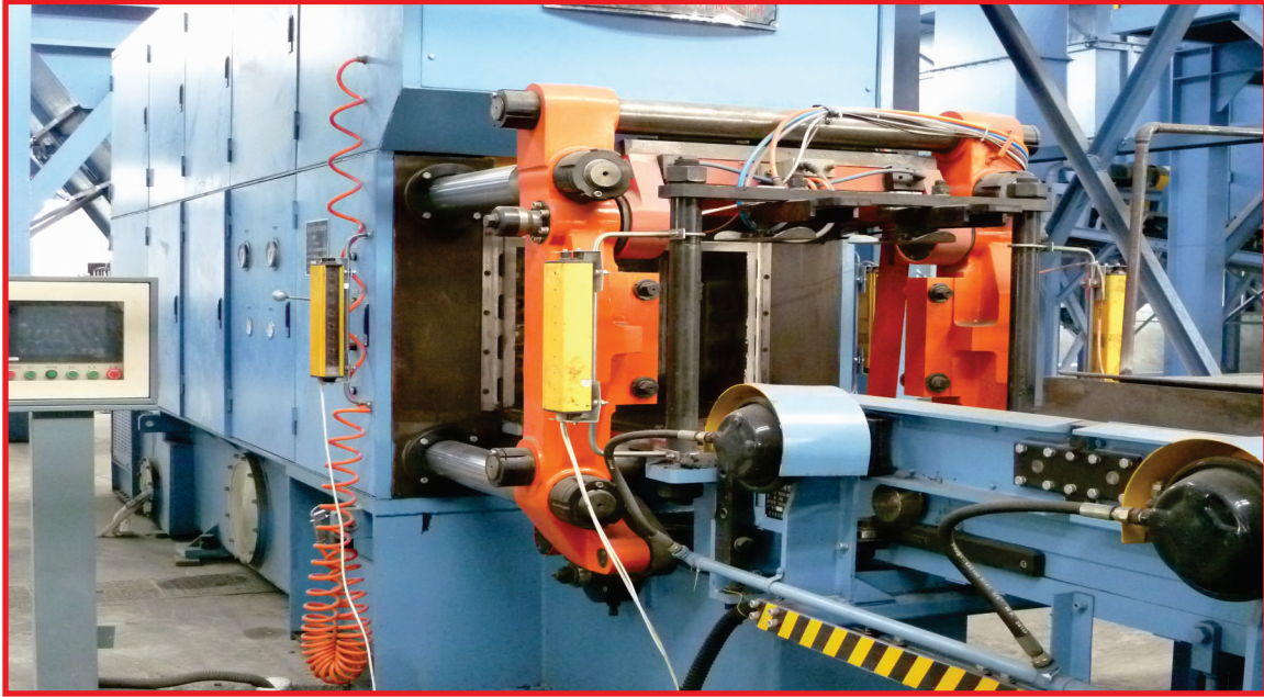
Z416B vertical moulding line
