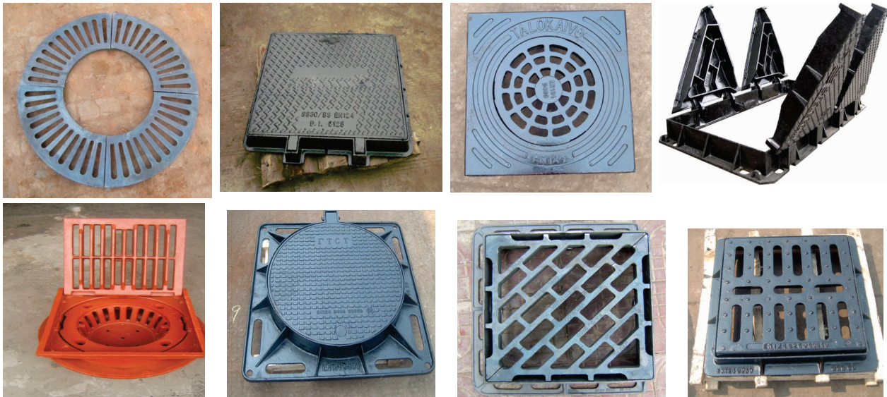
Manhole cover and grates as per EN124
