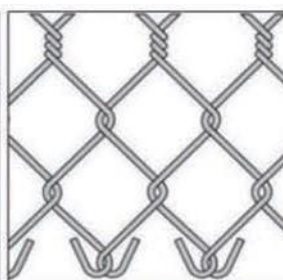
Twist & Knuckle
